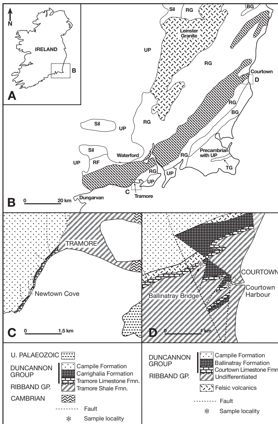
Fig. 1—Geological map of southeastern Ireland indicating position of the Duncannon Group (diagonally shaded) as well as Courttown and Tramore sampling localities.
