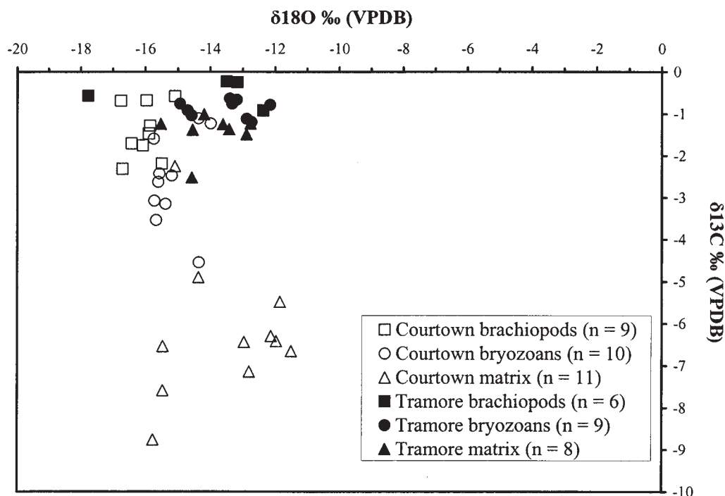
Fig. 2—Plot of \delta^{18}\text{O} vs \delta^{13}\text{C} for the brachiopod and bryozoan allochems and the matrix from the Courtown and Tramore Limestone Formations.
